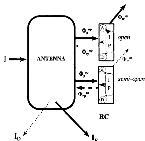
FIGURE 5 Energy trapping and fluorescence in PSII. I is the incident energy flux; \Phi_p , \Phi_{rp} , and \Phi_{tr} refer to probabilities for photochemical charge separation, radical pair recombination, and photochemistry ( Q_A reduction), respectively, with superscripts o and so referring to the open and semiopen state, respectively. The thickness of the arrows for \Phi_{tr} and \Phi_{rp} (dashed) is indicative for their respective magnitudes. Nonradiative (heat) losses in the reaction center are assumed to be relatively small in comparison with radical pair recombination and photochemistry. The diagonal oriented arrow points symbolize electron transfer at donor and acceptor side; radical pair recombination is symbolized with the horizontal arrow in the middle. Further explanations are in the text.
