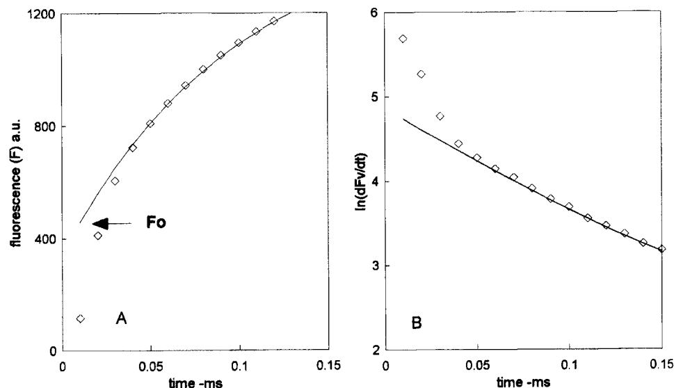
FIGURE 1 Fluorescence ( F ) data points of a dark-adapted Peperomia leaf collected in a Plant Efficiency Analyzer during the first 0.15 ms of illumination with 450 W\ m^{-2} light (open symbols in A) and a log plot of the first derivative of these data during the first ms of illumination (open symbols in B). Extrapolation of the slope in B in the time region 0.05–0.15 ms to the time domain <0.05 ms, where the fluorescence detector is limiting with a response time of \sim 0.03 ms, gives the fluorescence emission data in the 0.01–0.05-ms time domain (solid curves in A and B).
