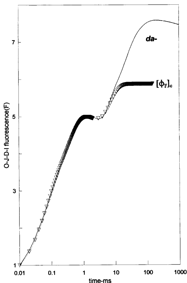
FIGURE 7 Simulated fluorescence induction curves (with symbols) for a dark-adapted Peperomia leaf. The fit parameters are given in Table 1. Further details are in the legend of Fig. 6 and in the text.
