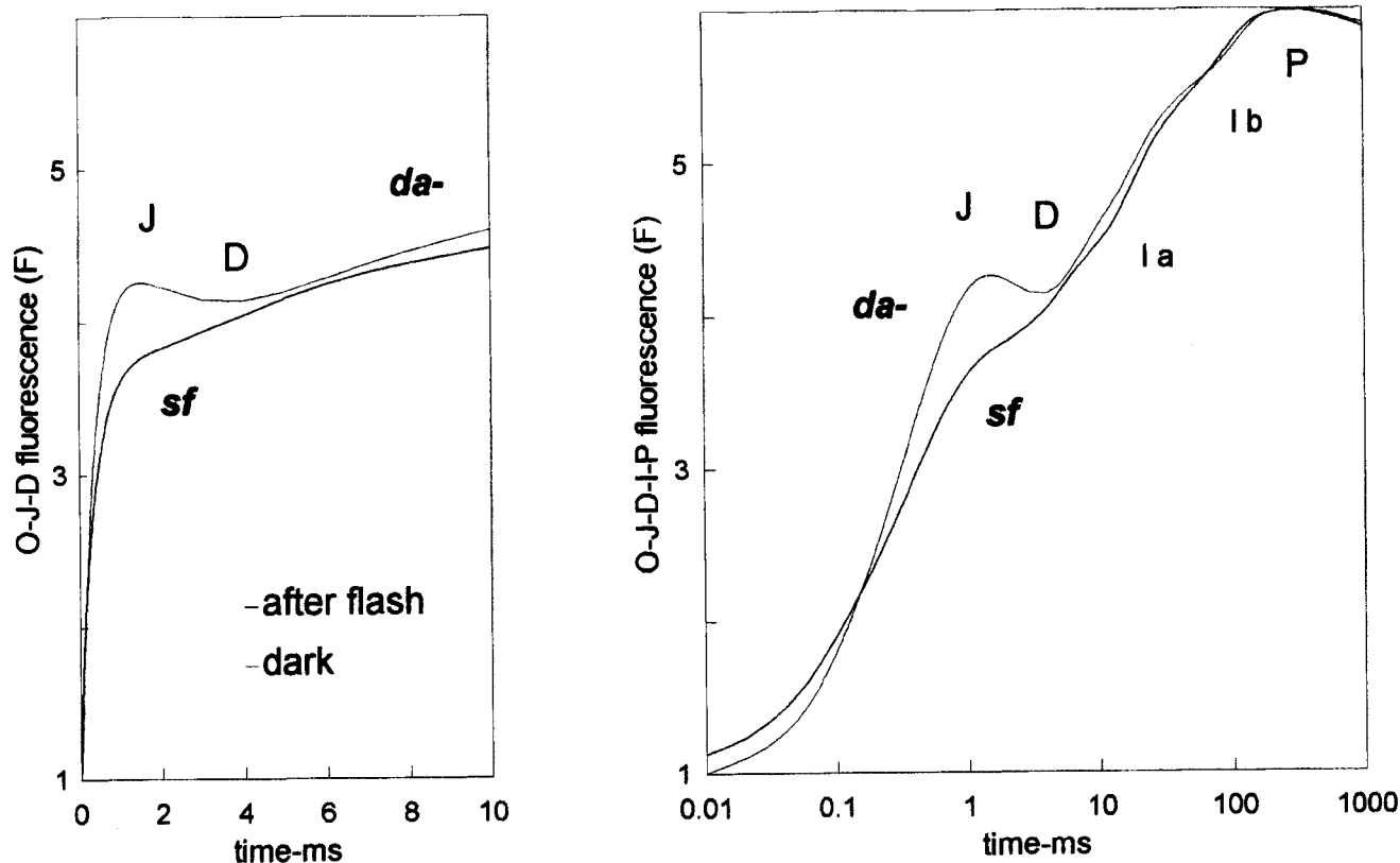
FIGURE 3 Fluorescence induction kinetics of a dark-adapted Chenopodium leaf before (da-) and 5 s after a single turnover saturating Xe flash (sf-). The curves have been normalized on the F_0 level ( F_0 = 1 ) of the da-leaf. Note the difference in F_0 and the different kinetics during the first 10 ms for the sf-leaf. Intensity of light was 600 \text{ W m}^{-2} . There is an intermediate hump in the J-I phase, which has been renamed J-I a -I b . See also legend of Fig. 5
