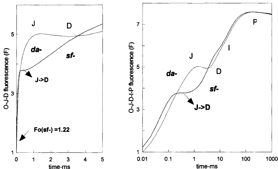
FIGURE 2 Fluorescence induction kinetics of a dark-adapted Peperomia metallica leaf before (da-) and 5 s after a single turnover pre-flash (sf-) plotted on a linear (left panel, but only for the first 5 ms) and a log time scale (right panel) with notations for the O-J-D-I- and P- levels. The curves have been normalized on the F_0 level ( F_0 = 1 ) of the da-leaf. Note the difference in F_0 and the different kinetics during the first 10 ms for the sf-leaf. Intensity of light was 450 \text{ W m}^{-2} . Noteworthy in the pre-flashed leaf is the \sim 22\% higher F_0 , the absence of the transient J-D phase of the fluorescence induction, the nearly constant fluorescence yield at the J level in the 0.1–1-ms time interval with F_J/F_0 \sim 0.7 , and coincidence with the da-curve above t \sim 20 \text{ ms} .
