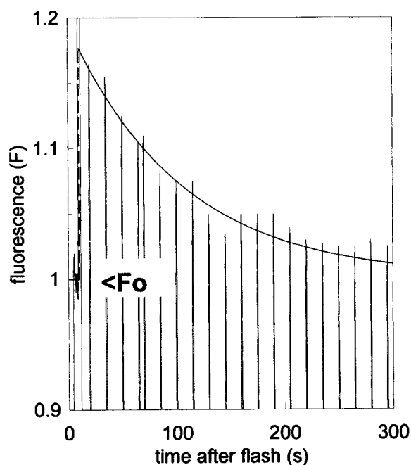
FIGURE 4 Fluorescence ( F ) yield (upward deflections) in a Peperomia leaf before ( F = F_0 = 1 ) and after a single turnover saturating pulse measured at 15-s intervals by low modulated light in a PAM fluorometer. The modulated excitation light beam was switched off for \sim 12 s every 15 s. The dashed vertical line marks the time at which the single turnover Xe flash was fired. The continuous curve is the exponential fit of \Delta F/F_0 (17.8%) with a relaxation time of 105 s.
