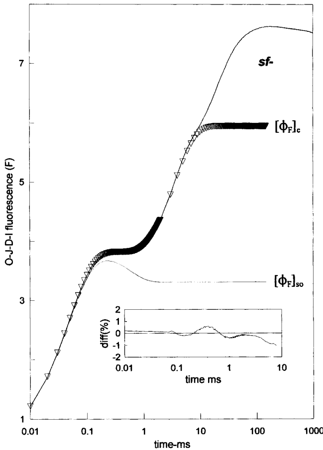
FIGURE 6 Simulated fluorescence induction curves (with symbols) for a dark-adapted Peperomia leaf after a single turnover pre-flash. Simulation was based on the presented model; the time 0 point of the simulated curve was taken as the 10- \mu s datapoint of the experimental curve (see Fig. 1). The fit parameters are given in Table 1. The lower thin curves in the time region between 0.01 and 5 ms represent the calculated accumulation of semiclosed centers in the absence of their slow conversion in the J-D-I phase. Insert: The difference between simulation and experimental datapoints on a percentage scale. Further details are in the text.
