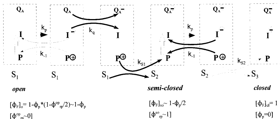
FIGURE 9 The three-state model of energy trapping in PSII under physiological (in vivo) conditions. Schematic visualization of six particular stages of the two-step closure of an open RC ( dashed rectangular ) in a multiturnover light pulse in a dark-adapted system ( S = S_1 ). Electron transfer to P^+ at the donor side after a first and second turnover causes transfer from S_1 \rightarrow S_2 \rightarrow S_3 . Open vertical and closed horizontal straight arrows represent exciton transfer (rate constant k_p ) and associated charge separation in the RC. The bent closed arrows mark electron transfer. The rate constants of the pertinent reactions are designated with k_q ( Q_A^- -reduction), k_1 (radical pair recombination), and k_{S1(2)} ( P^+ -reduction by Y_Z with S = S_1 and S_2 , respectively). Right- and left-oriented arrows symbolize the forward and backward transfer of an RC state, respectively. \Phi_F , \Phi_p , and \Phi_p are efficiencies for fluorescence emission, exciton transfer, and radical pair recombination, respectively. The thickness of an arrow is qualitatively related with the efficiency of the process or reaction it represents. Boxes 1, 4, and 6 (viewed from the left) represent the open, semiopen (-closed), and closed state, respectively. Boxes at position 2, 3, and 5 are transient closed states, which are transferred efficiently in the semiclosed state with transfer times in the submicrosecond time domain. These transient states are beyond the 10- \mu s time resolution of the fluorescence detection method (PEA, Hansatech) that has been used. The present scheme illustrates the situation at which the excitation rate ( \sim 100 \mu s ) ^{-1} is high as compared to the rate of Q_A^- -oxidation ( k_{-q} \sim (250 \mu s)^{-1} ). At lower excitation rates, the figure is representative for a system in the presence of DCMU; the lifetime of the semiopen state in the presence of DCMU is about 10 s (data not shown). The figure illustrates that at least two turnovers are required for stationary closure of an RC, the first and second step (semi- and full closure, respectively) of the closing mechanism occur with a large difference in trapping efficiency, and in the presence of DCMU the RCs of the system are transferred by one flash into a quasistationary semiclosed state with the initial fluorescence yield of the system equal to \Phi_F = [\Phi_F]_{so} = 1 - \Phi_p * (1 - \Phi_p^{op}/2) \sim 1 - \Phi_p/2 . Further explanations are in the text.
