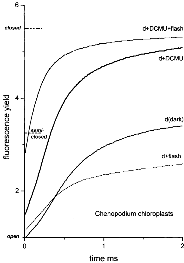
FIGURE 8 Changes in the fluorescence yield in a suspension of dark-adapted broken Chenopodium chloroplasts ( 20 \mu\text{g ml}^{-1} ) upon excitation with a 1-s light pulse of \sim 600 \text{ W m}^{-2} intensity in the absence ( lower two curves ) and presence ( upper two curves ) of 30 \mu\text{M} DCMU. In either case, the chloroplasts were preilluminated with a single turnover flash (indicated at the curves with “+flash”) or not. In the case of a pre-flash, the onset of the 1-s multiturnover light pulse was given 1.5–2 s after the pre-flash. The maximum fluorescence yield in the presence of DCMU was at 5.5. This level is indicated at the y axis with “closed.” The “semiclosed” level then is at 3.25, as indicated also. Note that the fluorescence level after a pre-flash in the presence of DCMU is somewhat below the level indicative for semiclosed RCs. (See further the text).
